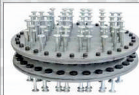
Pin Bearing
